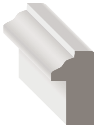
Stock Code MP2990BK1 (1544557) Dimensions \frac{3}{4} " x 1\frac{1}{4} " x 16' MP2990BK-08 (1544556)
