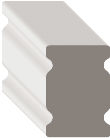
Stock Code MP558-07 (1544572) Dimensions 1 1/8" x 1 5/8" x 7'
