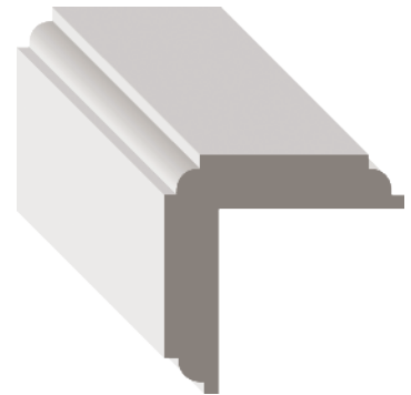
Stock Code MR012542 (1448287) Dimensions 1 1 / 8 " x 1 1 / 8 " x 8' O
